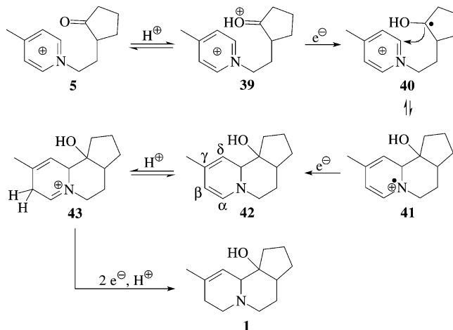
Scheme 11. Proposed mechanism of the cathodic cyclisation, shown for the synthesis of indolizidine 1 from the pyridinium salt 5
