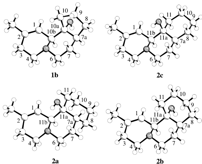
Figure 1. Crystal structures of the quinolizidines 1b and 2a–2c
