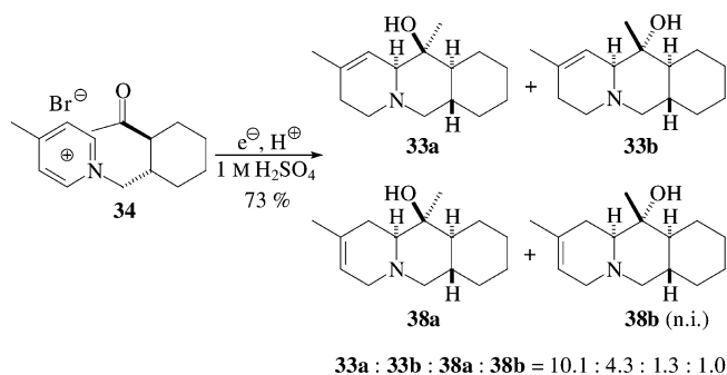
Scheme 10. Electrolysis of 34 to afford the [b]-annelated quinolizidines 33 and 38
