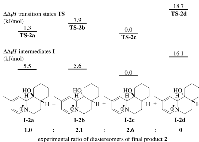
Scheme 13. Calculated \Delta\Delta_f H values of the transition states TS and the cyclised intermediates I for the reduction of the salt 6 to the quinolizidine 2
