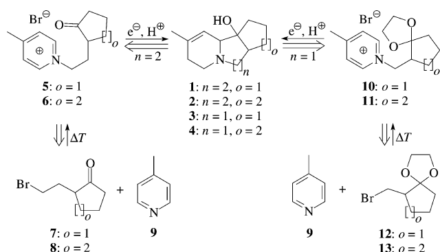
Scheme 1. Retrosynthetic analysis of the [a]-annelated indolizidines and quinolizidines 1–4
