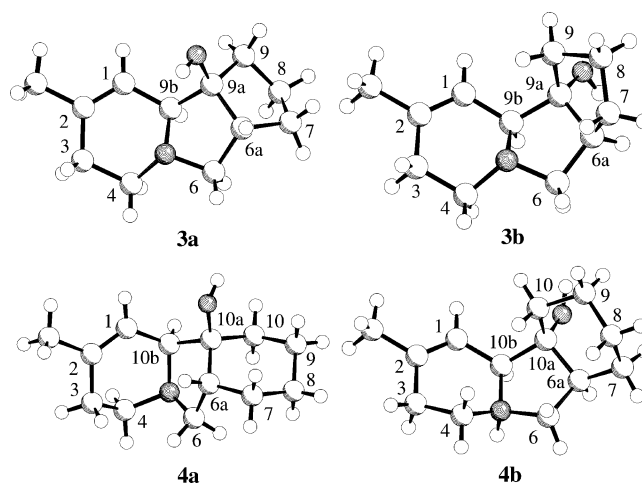
Figure 2. Crystal structures of the indolizidines 3a , 3b , 4a and 4b
