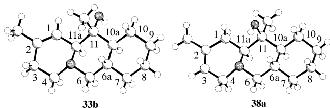
Figure 3. Crystal structures of the [b]-annelated quinolizidines 33b and 38a
