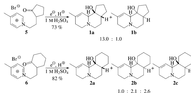
Scheme 8. Electrolysis of 5 and 6 to afford the quinolizidines 1 and 2
