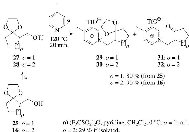
Scheme 5. Synthesis of the cyclisation precursors for the indolizidines from 25 and 16 via triflates
