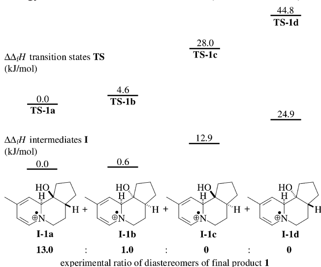
Scheme 12. Calculated \Delta\Delta_f H values of the transition states TS and the cyclised intermediates I for the reduction of the salt 5 to the quinolizidine 1
