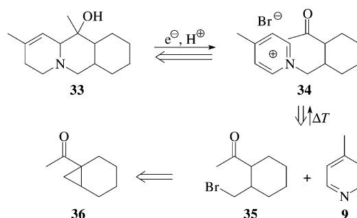
Scheme 6. Retrosynthetic analysis of the cyclohexa[ b ]quinolizidine 33
