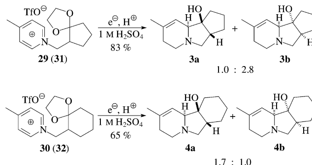
Scheme 9. Electrolysis of 29 and 30 to afford the indolizidines 3 and 4
